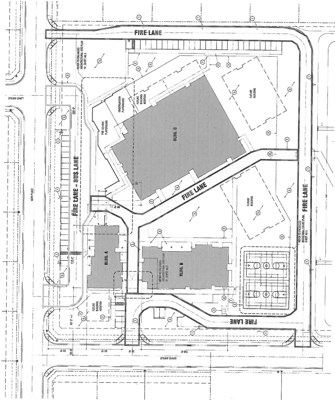
ENLARGED ARCHITECTURAL SITE PLAN SCALE 1" = 30'-0"
